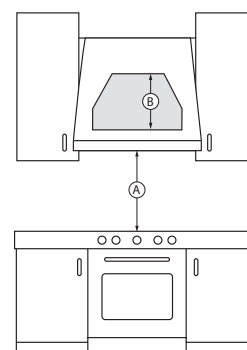
A. Installation height above the cooking surface 24-30" B. The distance from bottom of range hood to top of range hood: 11"
